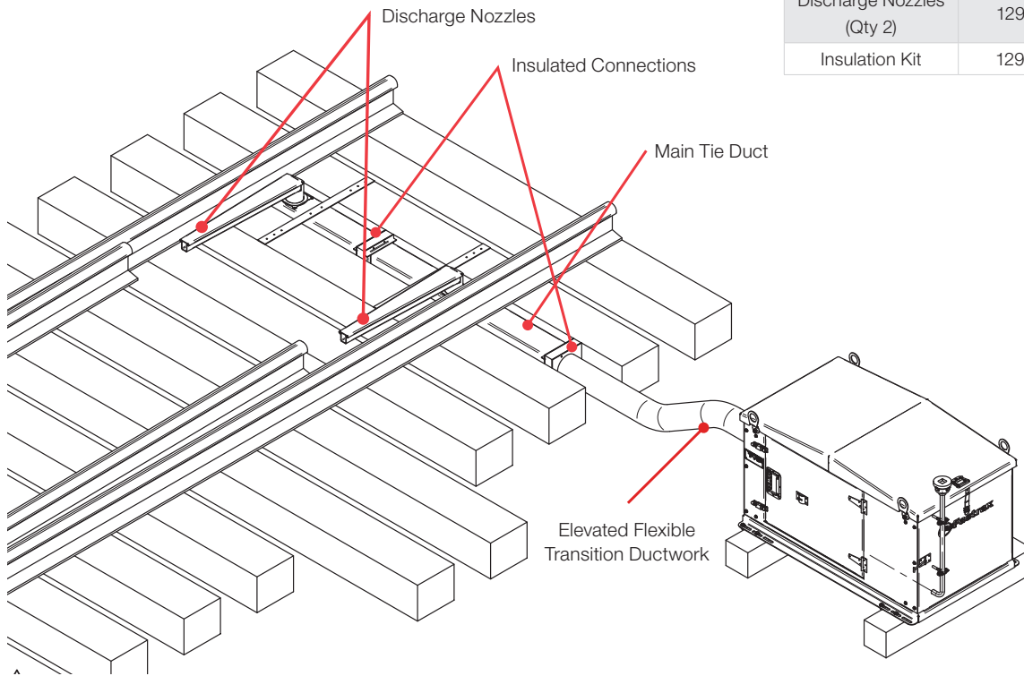
Figure 19 – Duct Package Assembly
